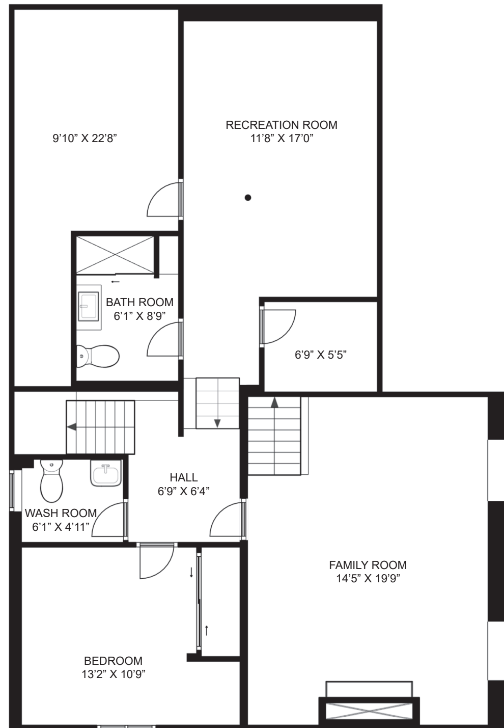
LOWER FLOOR
