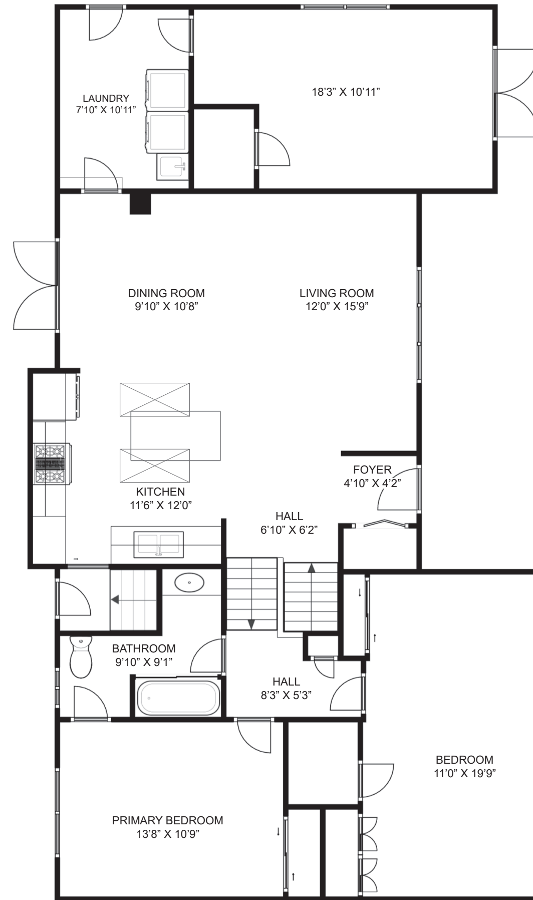
MAIN FLOOR
