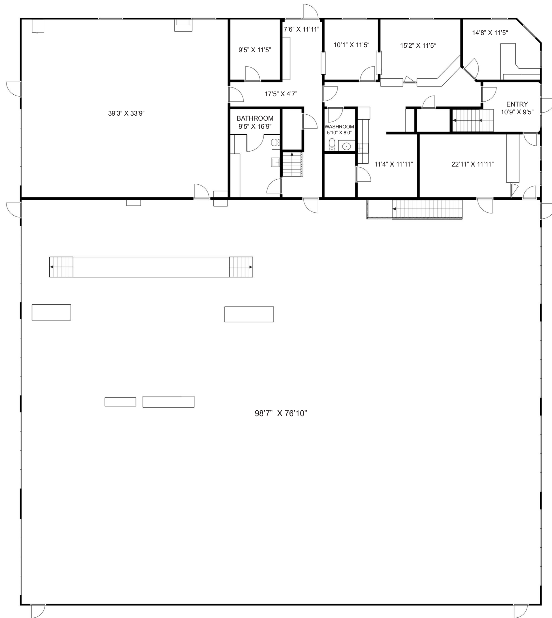
MAIN FLOOR
