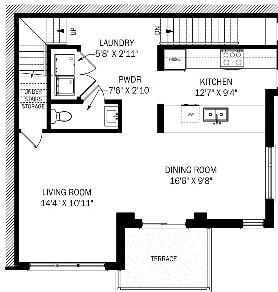
CEILING HEIGHT 9'0" MAIN LEVEL - 748 SQUARE FEET
