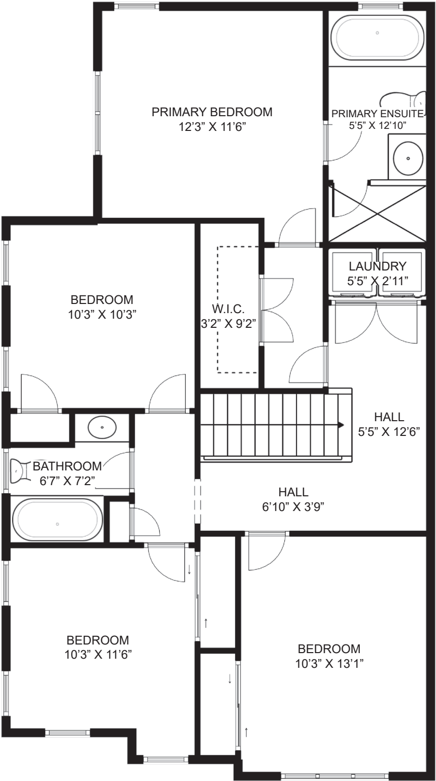
UPPER FLOOR
