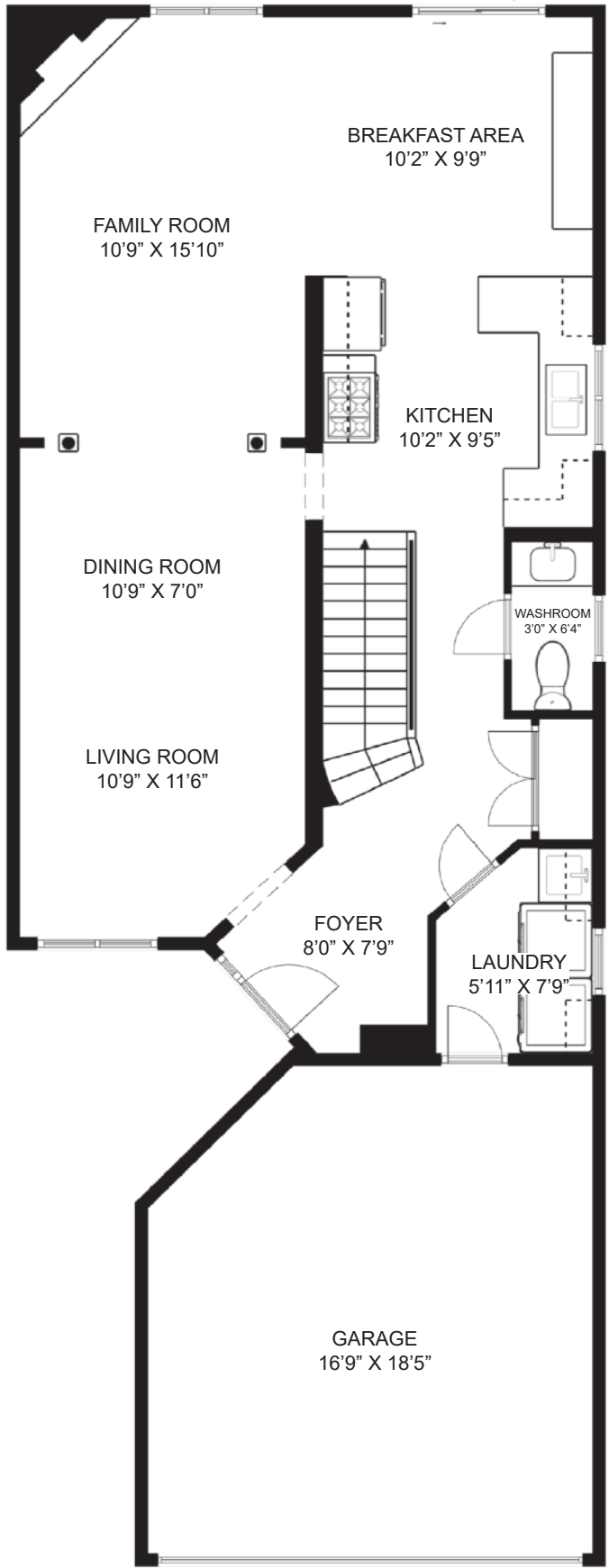
MAIN FLOOR
