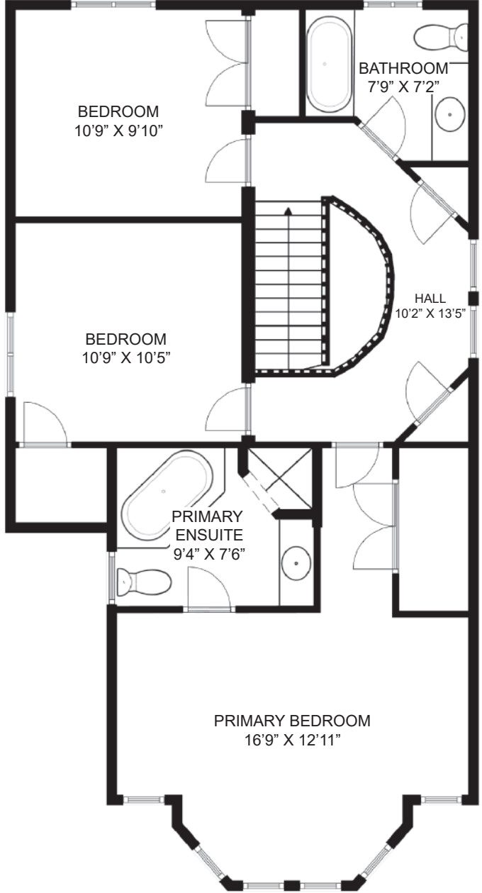
UPPER FLOOR
