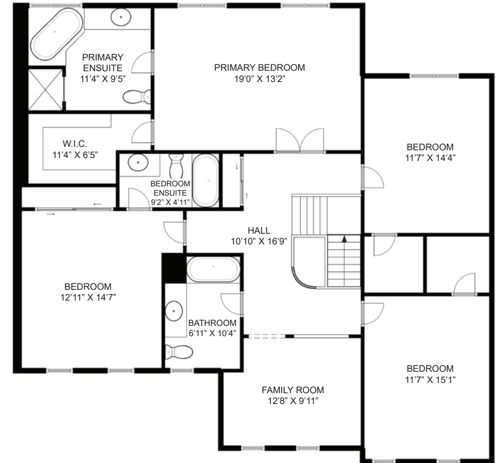
UPPER FLOOR 1,643 sq.ft.
