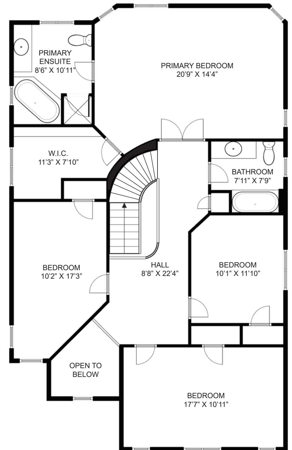
UPPER FLOOR
